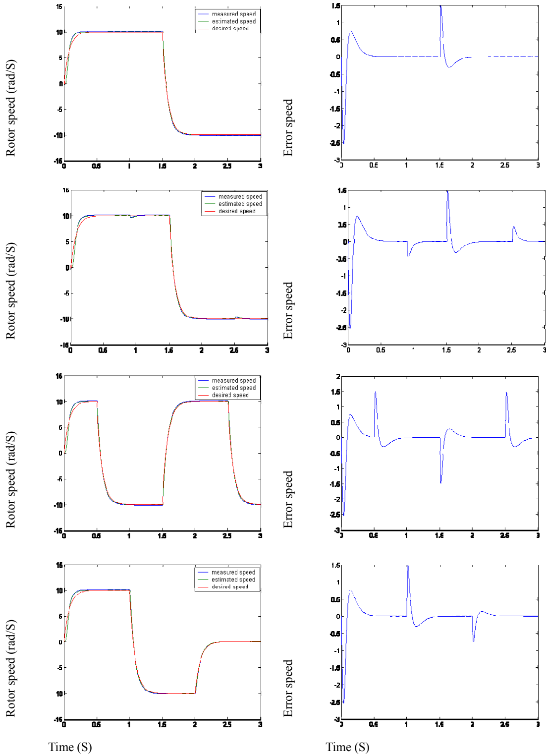
Fig. 6: Simulated speed response for step varying of the reference speed
