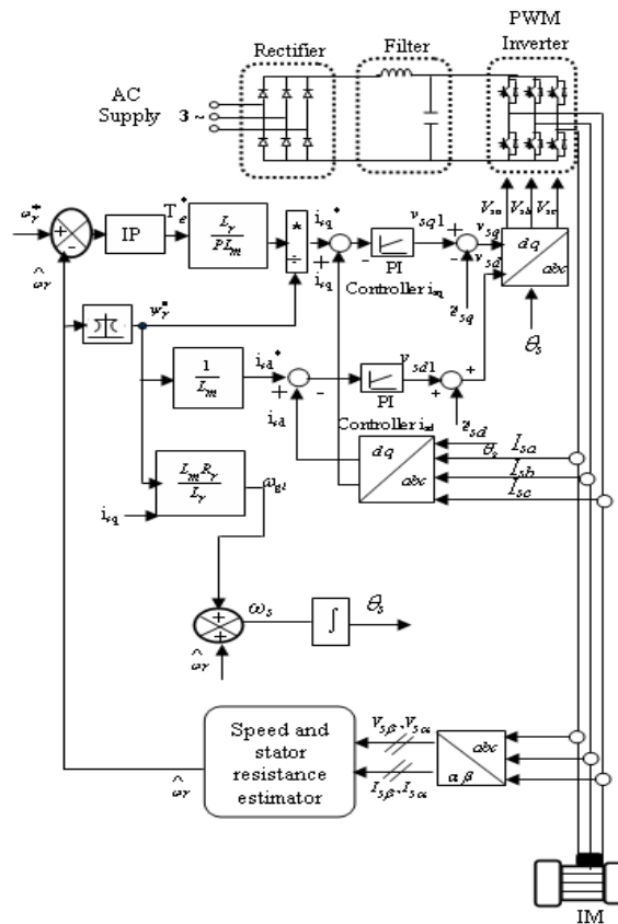
Fig. 4: Block diagram of sensorless (IFOC) with stator resistance tuning of induction motor drive system.
