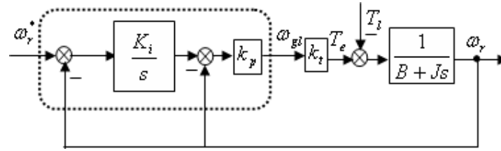
Fig. 1: Bloc diagram of IP speed controller
