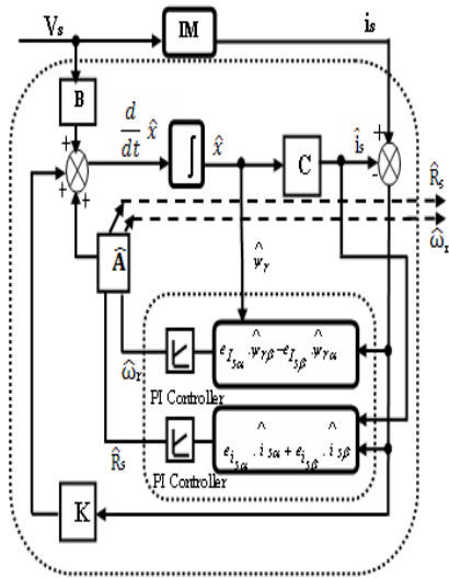
Fig. 3: Block diagram of simultaneous estimation of rotor speed and stator resistance
