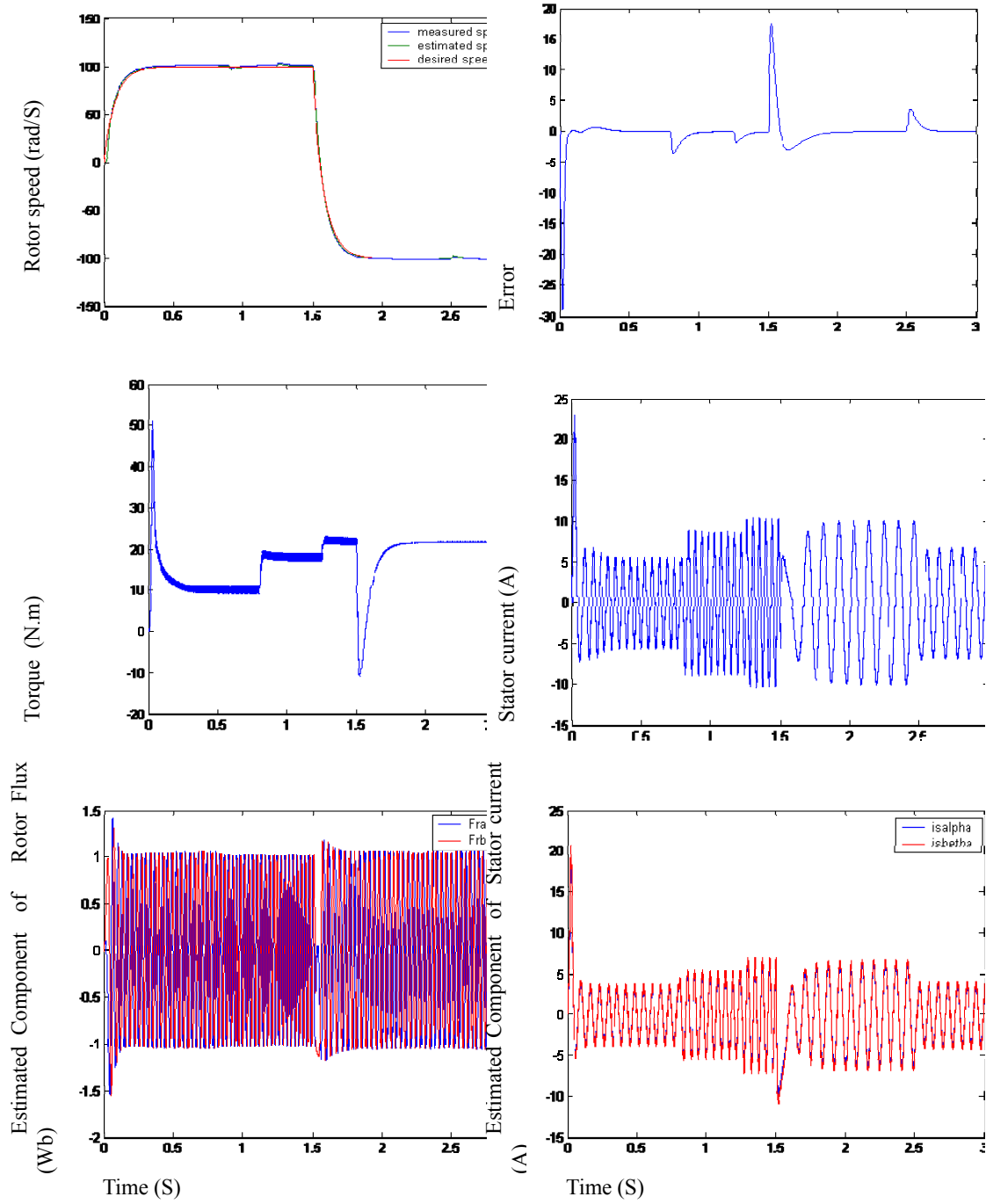
Fig. 5: Performances of speed control using an L O proposed with a speed reverse and under load change.
