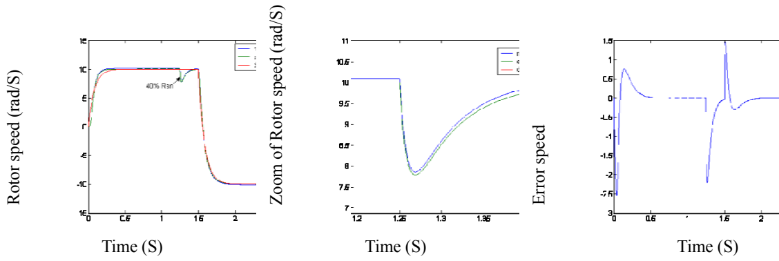
Fig. 7: Simulation results of the speed estimation with stator resistance increased sharply by 40% from R_{sn}
