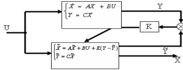
Fig. 2: structure of Luenberger Observer
