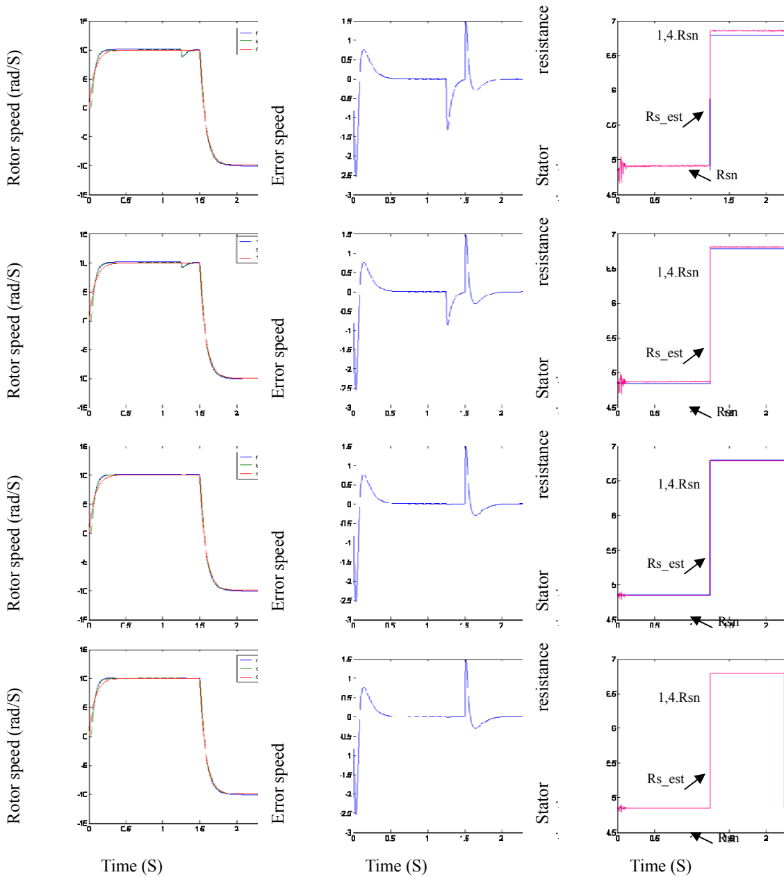
Fig. 8: Simulation results of the speed and stator resistance estimation
