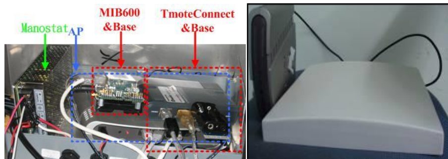
Fig. 4: Wireless AP with two gateways and antenna
