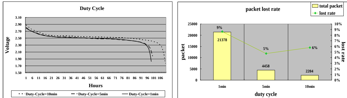
Fig. 9: (a) duty cycle and (b) packet lost
