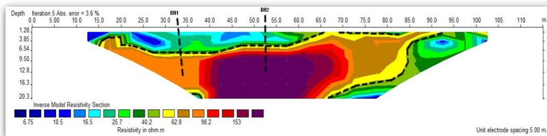
Fig. 4: Electrical resistivity pseudo-section profiles (1)
