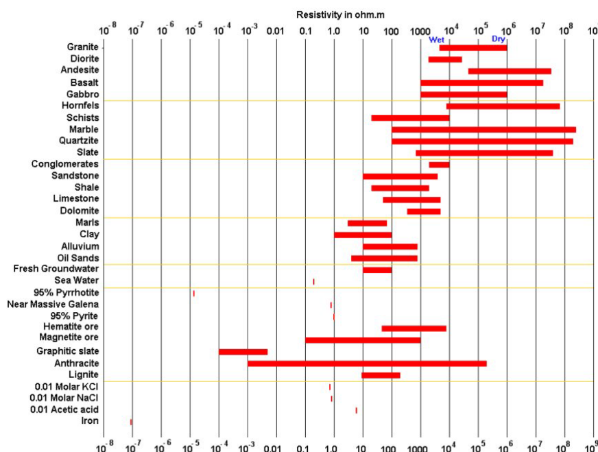
Fig. 1: Ground resistivity material
