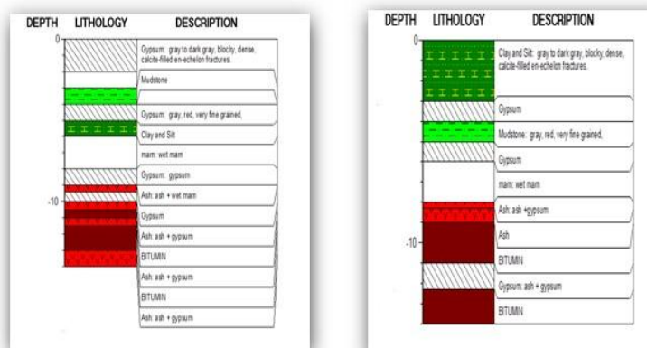
Fig. 7: Boreholes BH3 and BH4
