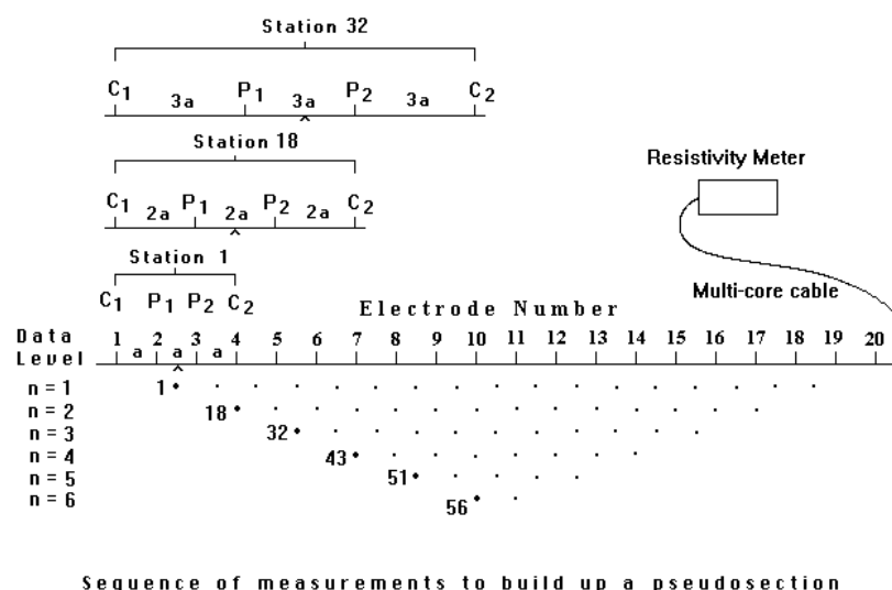
Fig. 1: Ground resistivity material
