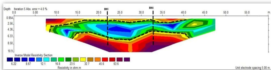
Fig. 5: Electrical resistivity pseudo-section profiles (2)
