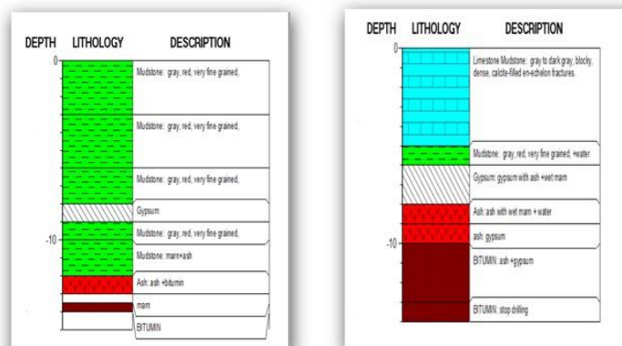
Fig. 6: Boreholes BH1 and BH2
