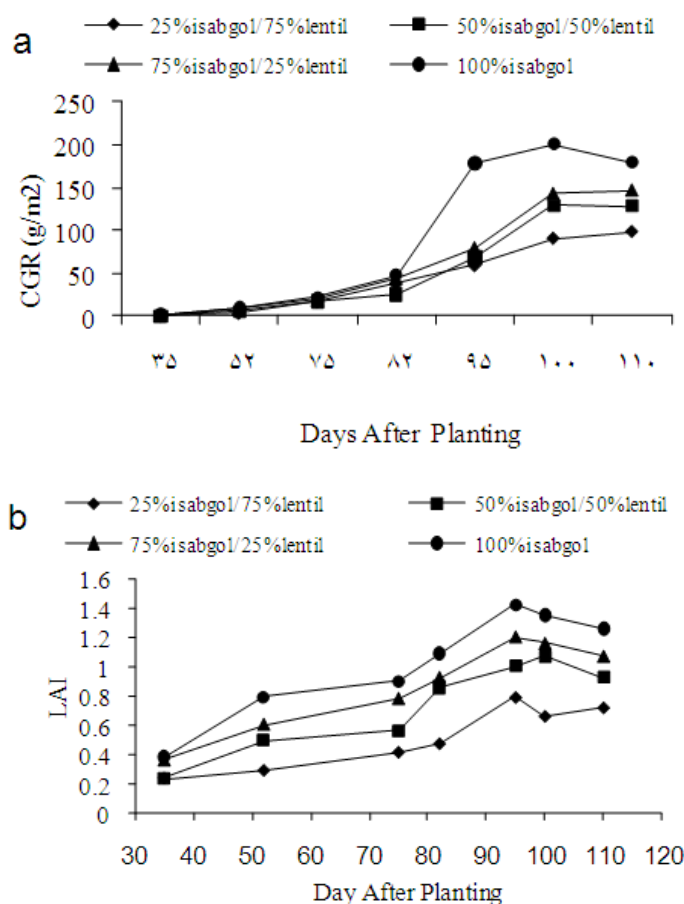
Fig. 1: Effects of cropping systems on (a) CGR and (b) LAI of isabgol plants during growth season
